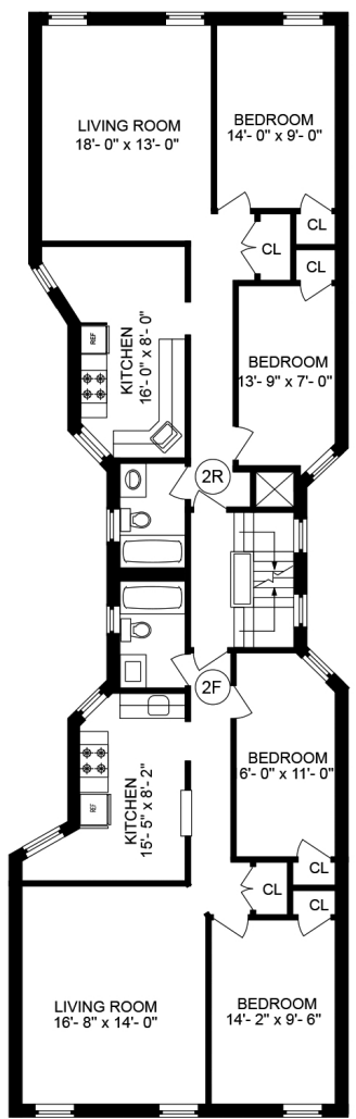
SECOND FLOOR
